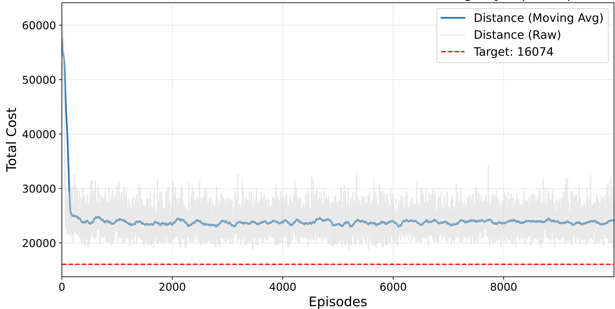
Final HYPERBAND GP Masked AutoRL-SOP Training - ry48p.2.sop
